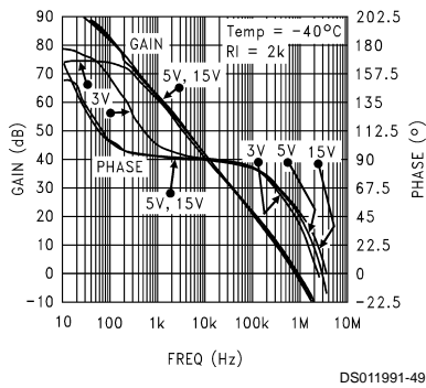
Open Loop Frequency Response @ -40^\circ C
