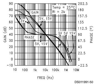
Open Loop Frequency Response @ 25^\circ C
